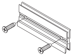
450VG640 4" REVERSABLE STOOL TRIM CLIP PACKAGE (TRIFAB 400 & TRIFAB VG 450)
