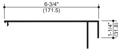
069268 6-3/4" STOOL TRIM
