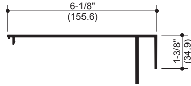
069267 6-1/8" STOOL TRIM
