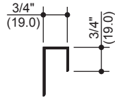
069263 GYPSUM BOARD TRIM
