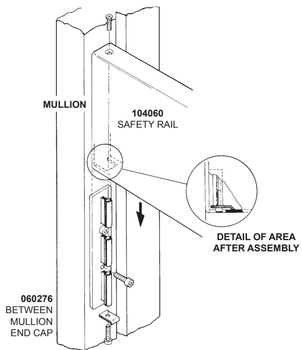
RAILING MOUNTED BETWEEN MULLIONS
