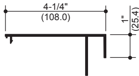
069265 4-1/4" STOOL TRIM
