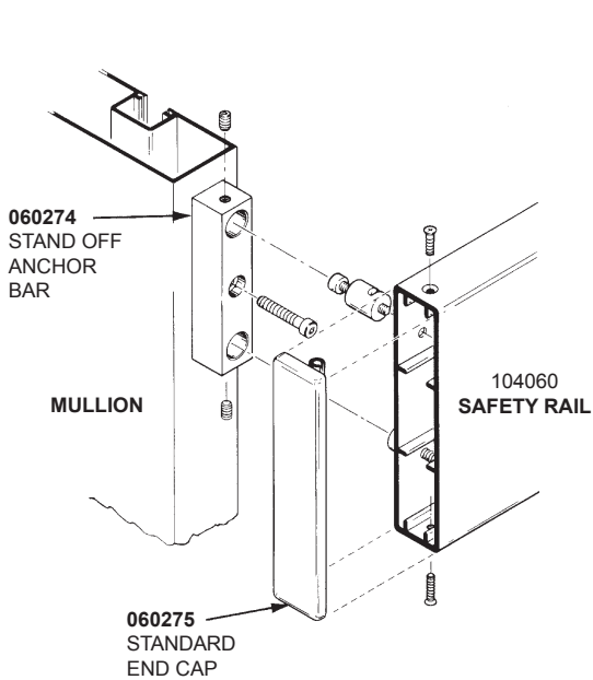
RAILING MOUNTED ON FACE OF MULLION
