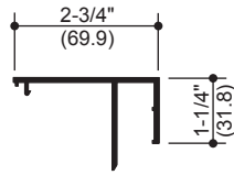
069264 2-3/4" STOOL TRIM
