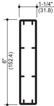
104060 SAFETY RAIL
